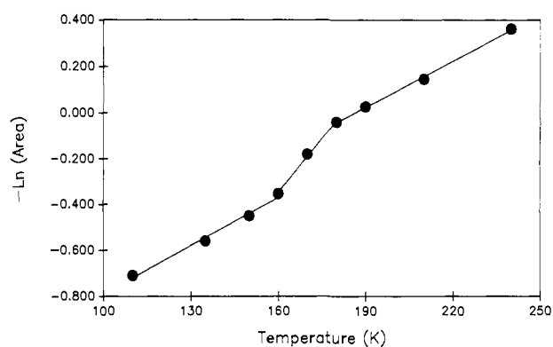
Figure 9. Plot of minus the natural logarithm of the base-line-normalized spectral areas versus temperature evaluated from the ^{57}Fe Mössbauer spectra for a sample of [^{57}Fe_2^{III}Mn^{II}O(O_2CCH_3)_6(py)_3](py) doped into [Mn_3O(O_2CCH_3)_6(py)_3](py) . Error bars are contained within the size of the symbols.
