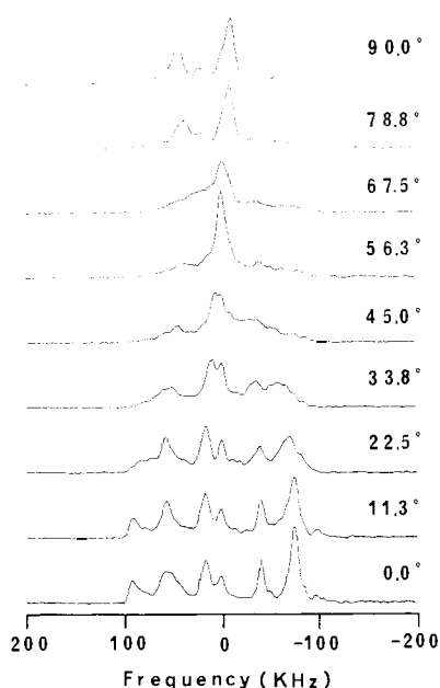
Figure 8. ^2H NMR spectra for magnetically oriented microcrystalline sample of [Mn_3O(O_2CCH_3)_6(C_5D_5N)_3](C_5D_5N) embedded in an eicosane matrix at 275 K. The angle between the magnetic field and the principal axis of the susceptibility tensor (i.e., c axis) is given for each spectrum.
