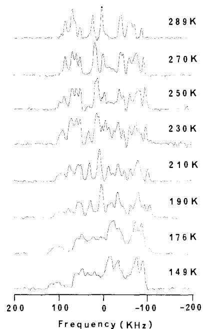
Figure 6. Variable-temperature ^2\text{H} NMR spectra for a \sim 1.5 \times 1.5 \times 1.5 mm single crystal of [\text{Mn}_3\text{O}(\text{O}_2\text{CCH}_3)_6(\text{C}_5\text{D}_5\text{N})_3](\text{C}_5\text{D}_5\text{N}) embedded in hexadecane and oriented so that the magnetic field is parallel to the crystallographic c axis.
