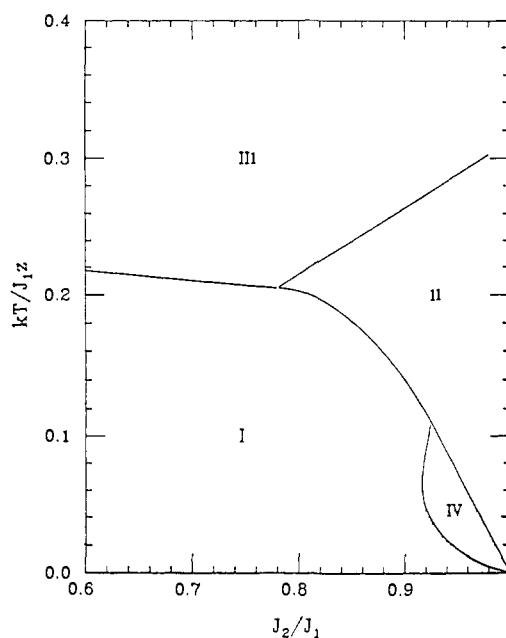
Figure 10. Phase diagram calculated by Stratt and Adachi 22 employing a mean field theory to account for the phase transitions in mixed-valence M_3O complexes, which crystallize in the R32 space group. The vertical axis is temperature plotted in units of J_1 z/k , where k is the Boltzmann constant, z is the number of M_3O complexes surrounding each M_3O complex, and J_1 is the interaction energy of two neighboring complexes, both of which are distorted parallel to each other. The horizontal axis is the ratio of the antiferrodistortive ( J_2 ) to the ferrodistortive ( J_1 ) coupling, where J_2 is the interaction energy for two neighboring complexes, one of which is distorted and the other is undistorted.
