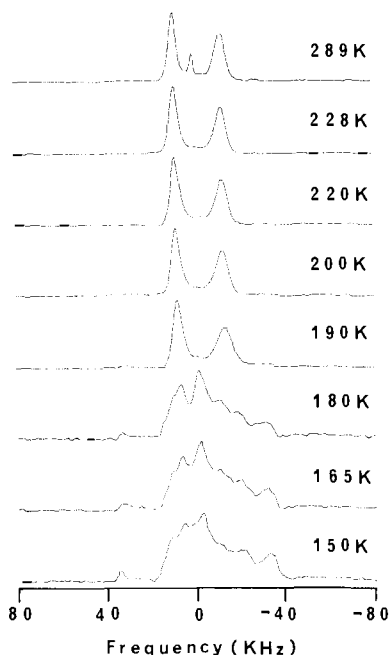
Figure 5. Variable-temperature ^2\text{H} NMR spectra for a \sim 1.5 \times 1.5 \times 1.5 mm single crystal of [\text{Mn}_3\text{O}(\text{O}_2\text{CCD}_3)_6(\text{py})_3](\text{py}) embedded in hexadecane and oriented so that the magnetic field is parallel to the crystallographic c axis.
